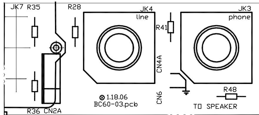
Output Board
